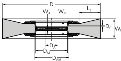
Wheel brushes
