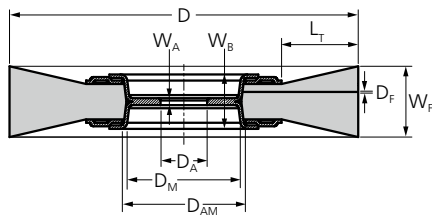
Wheel brushes
