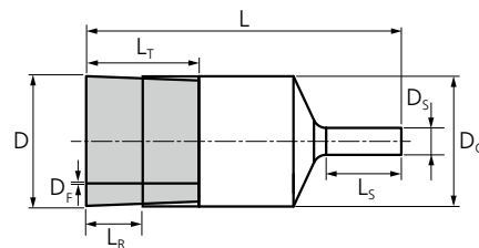
End brushes
